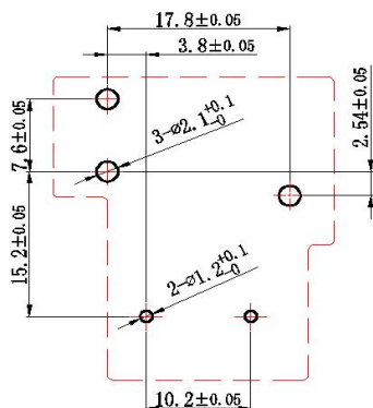
线路板孔位图 (底视图) PCB LAYOUT (BOTTOM VIEW)
