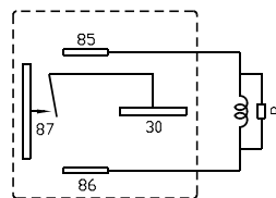
带电阻型 With resistor
