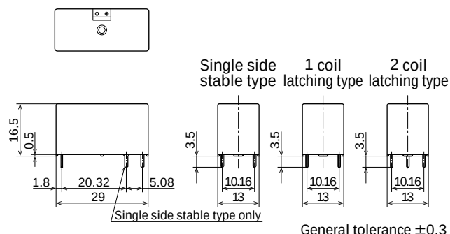
External dimensions
