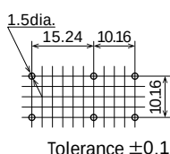
Recommended PC board pattern (BOTTOM VIEW)
