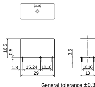
External dimensions
