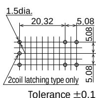
Recommended PC board pattern (BOTTOM VIEW)
